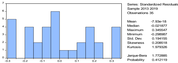
Figure 1: Normality test result
